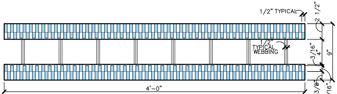
2 TOP / BOTTOM VIEW (REVERSIBLE) SCALE: 1 1/2" = 1'-0"
