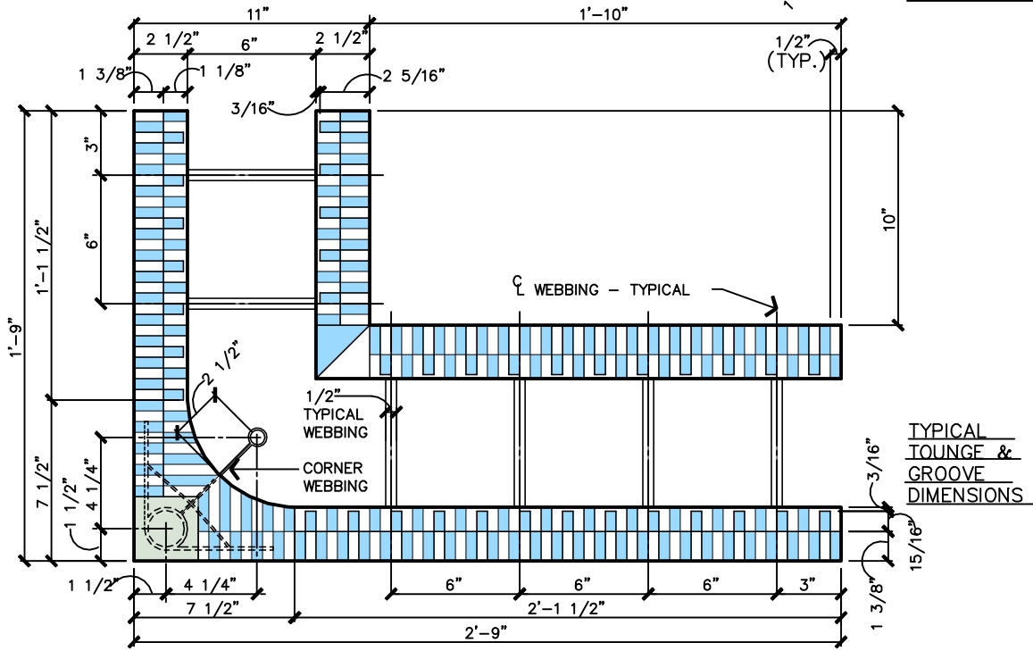
1 02 90° REVERSIBLE CORNER TOP / BOTTOM VIEW SCALE: 1 1/2" = 1'-0"
