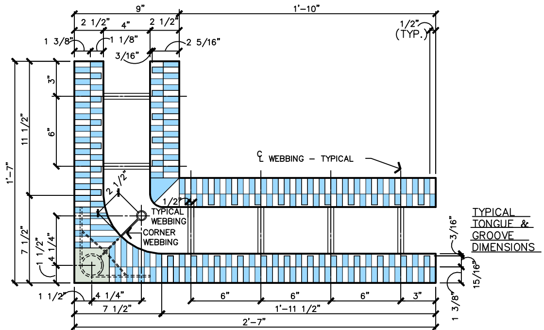
90° REVERSIBLE CORNER TOP / BOTTOM VIEW
