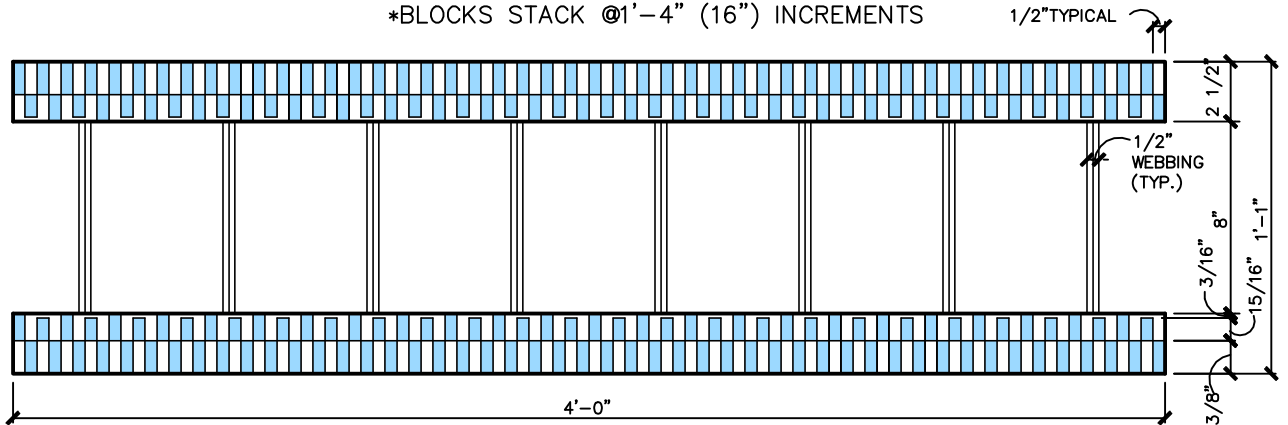
2 TOP / BOTTOM VIEW (REVERSIBLE) SCALE: 1 1/2" = 1'-0"
