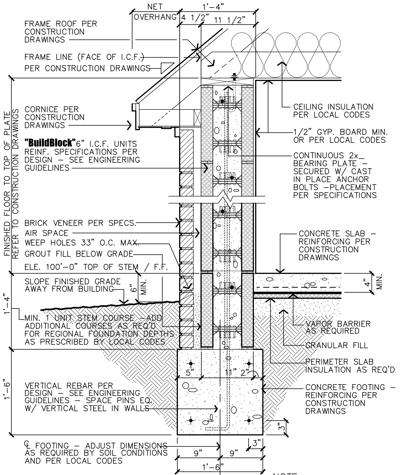
1 TYPICAL WALL SECTION 06 SCALE: 1" = 1'-0"
