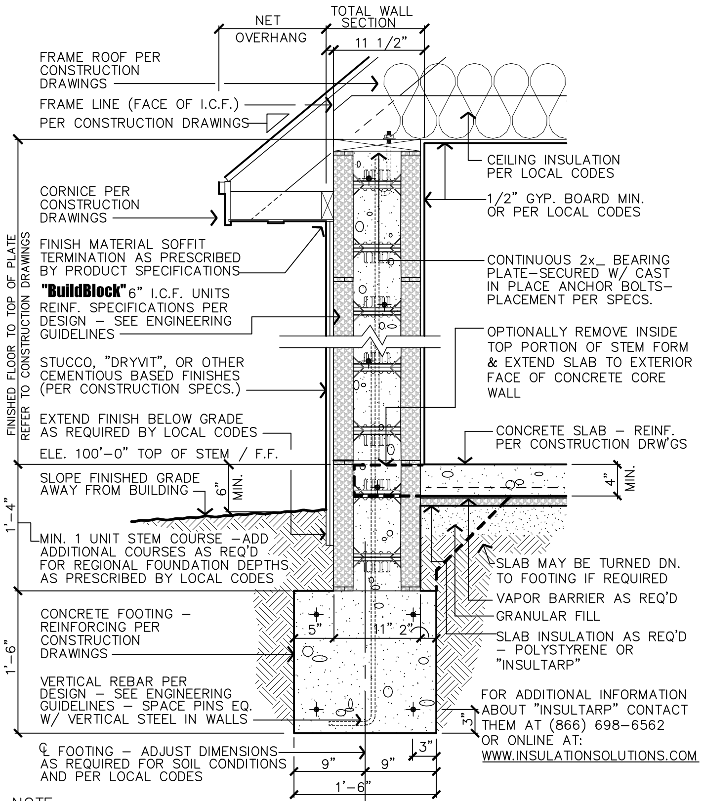
1 07 TYPICAL WALL SECTION SCALE: 1" = 1'-0"
