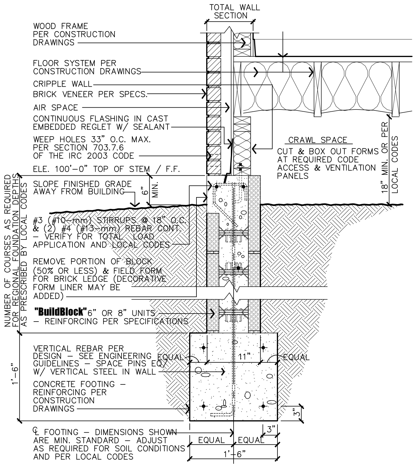
1 FOUNDATION DETAIL 10 SCALE: 1" = 1'-0"
