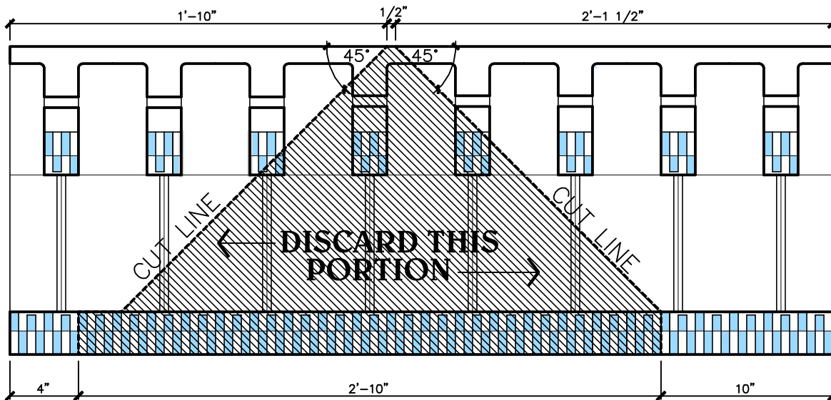
3 CUTTING DIAGRAM (TOP VIEW FULL BLOCK) SCALE: 1 1/2" = 1'-0"
