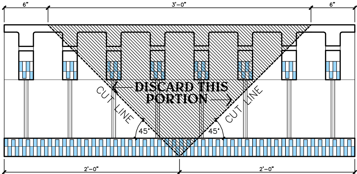
② CUTTING DIAGRAM (TOP VIEW FULL BLOCK) 44 SCALE: 1 1/2" = 1'-0"
