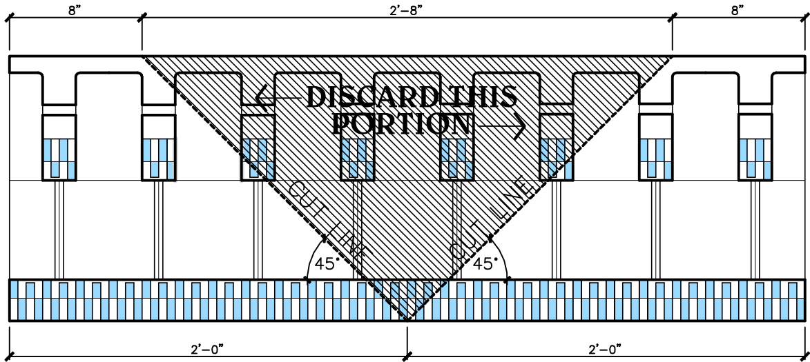
2 44a CUTTING DIAGRAM (TOP VIEW FULL BLOCK) SCALE: 1 1/2" = 1'-0"
